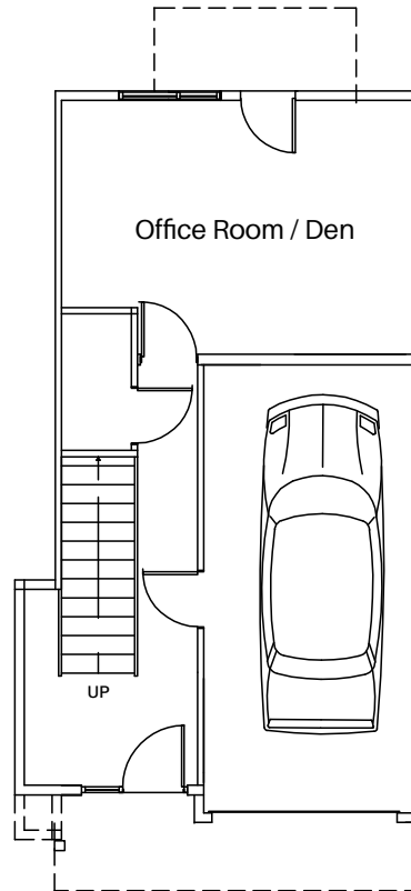
LOWER FLOOR AREA 365 SQ.FT. GARAGE 226 SQ.FT.
